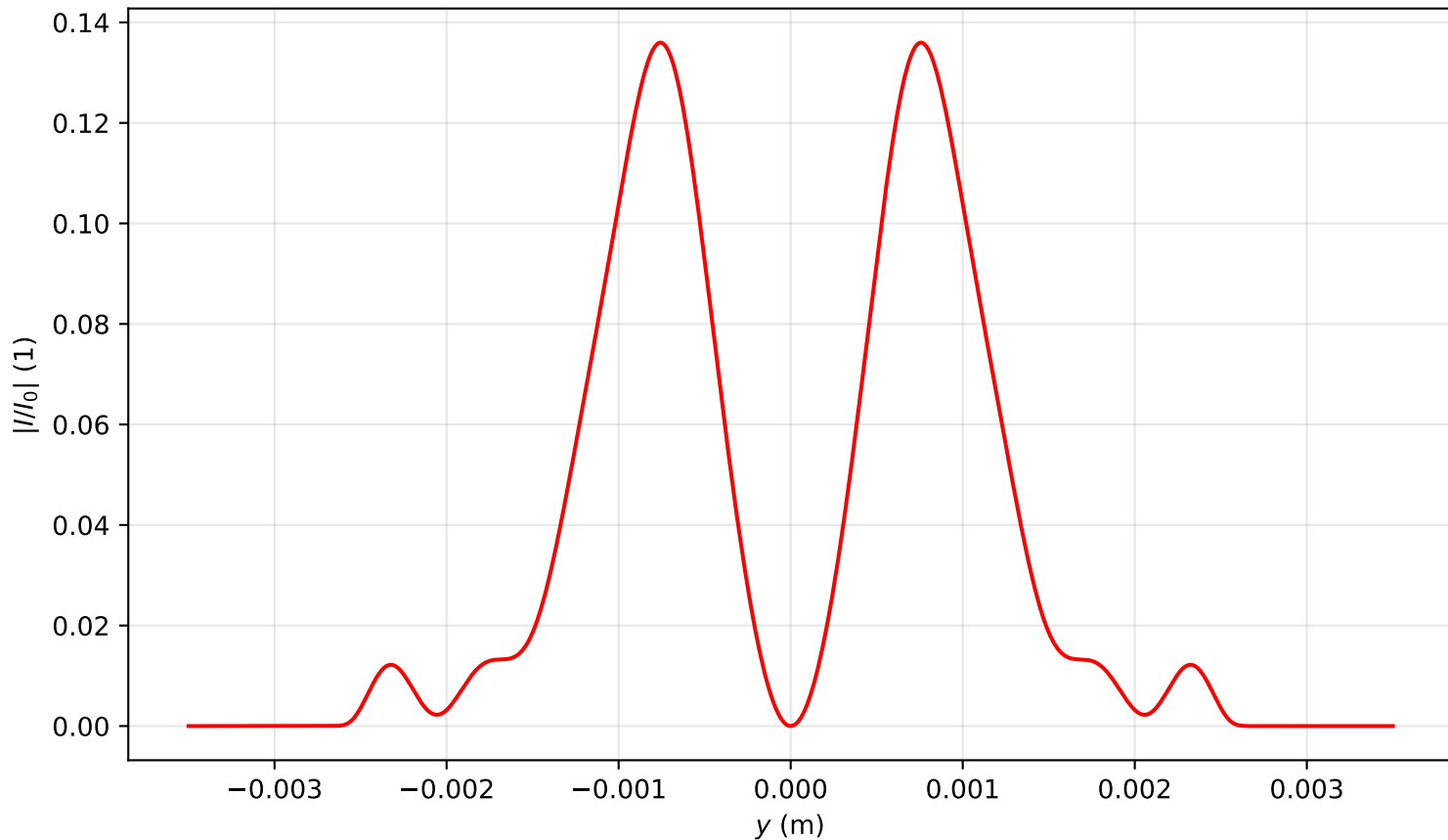
Intensity profile I(x = 0, y, z = 3.264)/I_0 , \text{Pin}=4.0\text{Pcr} , artificial time
